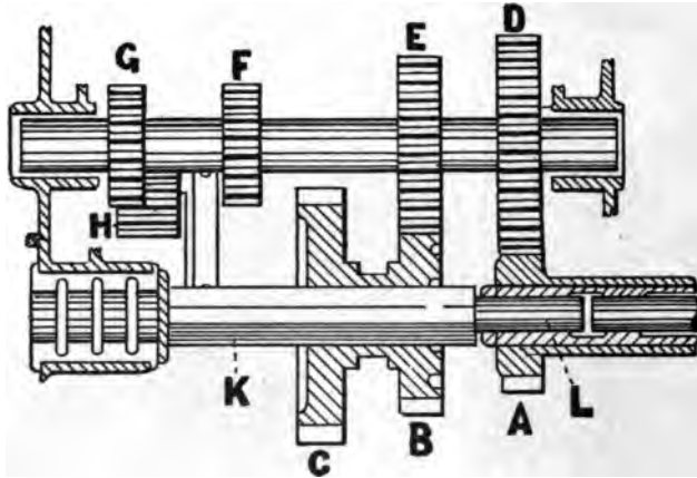
FIG. 252.—Diagram of the Decauville Transmission Gear. A is the spur pinion at the end of the clutch shaft; B and C, spurs on the sliding sleeve; D, E, F, G, spurs keyed to the second motion shaft; H, the reverse pinion, constantly in mesh with G, and giving the reverse when in mesh with C also; K, the square portion of the drive shaft; L, portion of same journaled into the clutch shaft.
